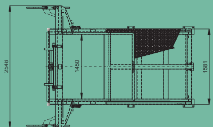
contour romsky joko SP50LR
