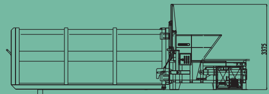
contour romsky joko SP50LR
